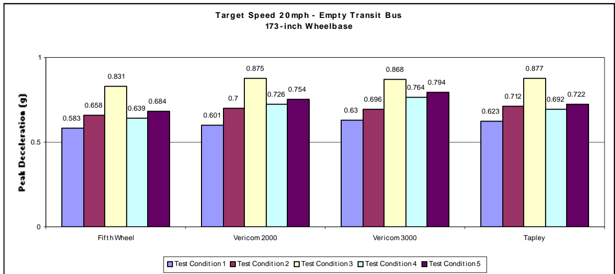
Figure 2 – Medium wheelbase transit bus
